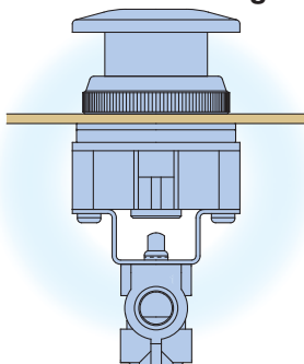
Panel mounting
