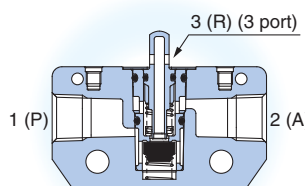
Side ported
