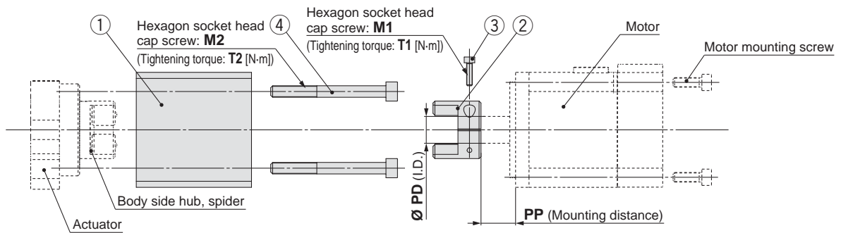
Motor flange details
