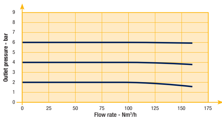
Flow Curve 1"
