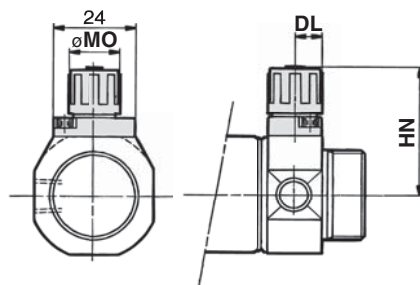
Locking type manual release: Suffix L
