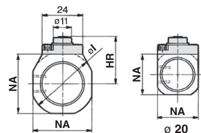
Non-locking type manual release: Suffix N
